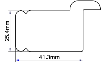
41.3mm D-Mould Stile
