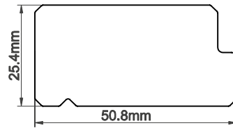
50mm Plain Rebate Stile
