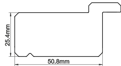
50mm Plain D-Mould Stile
