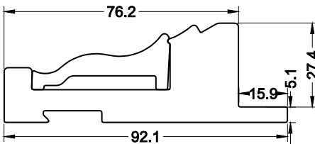
RIDGE DECO FRAME
