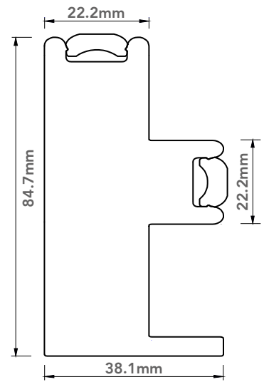
Double Insert F Frame 84mm
