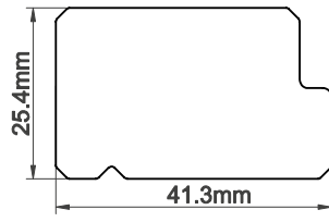
41.3mm Plain Rebate Stile
