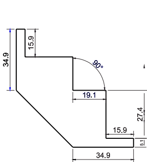
(Deco Frame) 32mm
