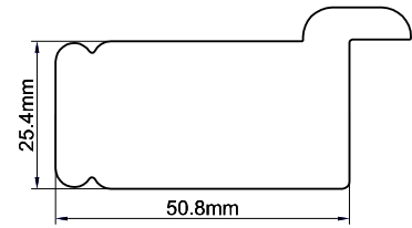
50.8mm D-Mould Stile
