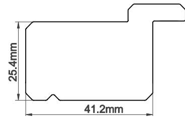
41.3mm Plain D-Mould Stile
