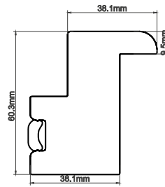
BULLNOSE Z DEEP W/INSERT
