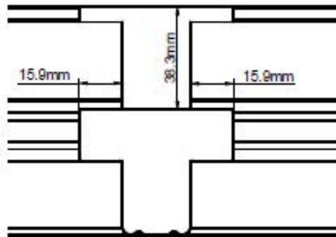
Double Insert F Frame 84mm
