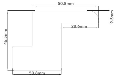
BULLNOSE Z FRAME
