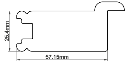
57mm D-Mould Stile
