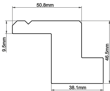
SERRATE Z FRAME
