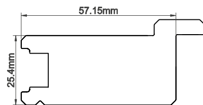
57mm Plain D-Mould Stile
